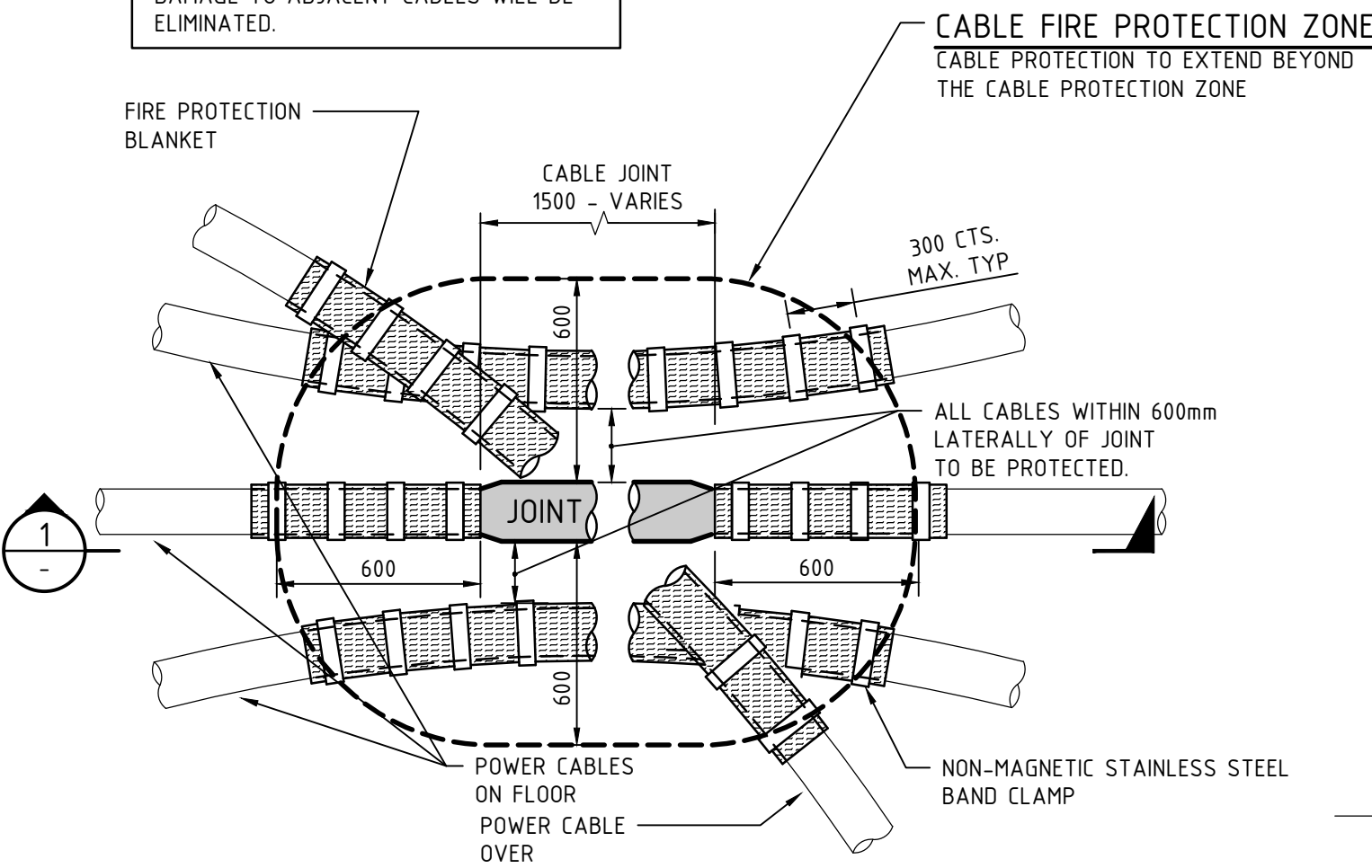
PLAN AT CABLE ON FLOOR
