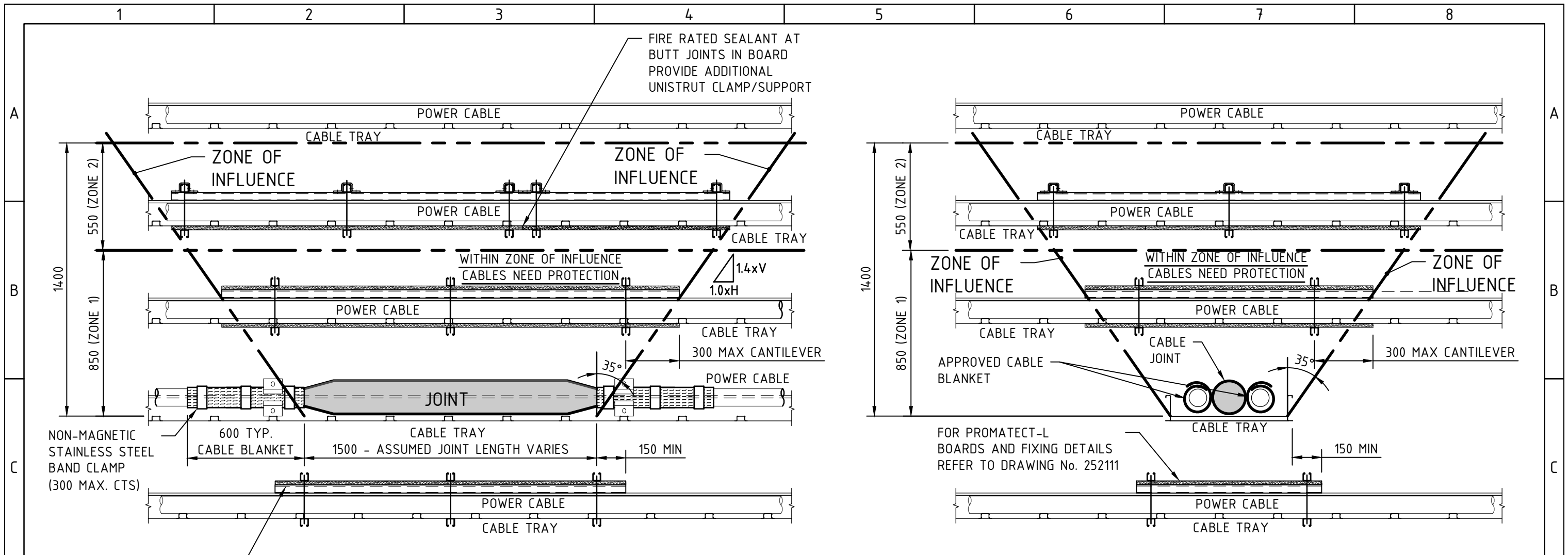
AT CABLE JOINT WHERE PARALLEL TO ADJACENT CABLES
