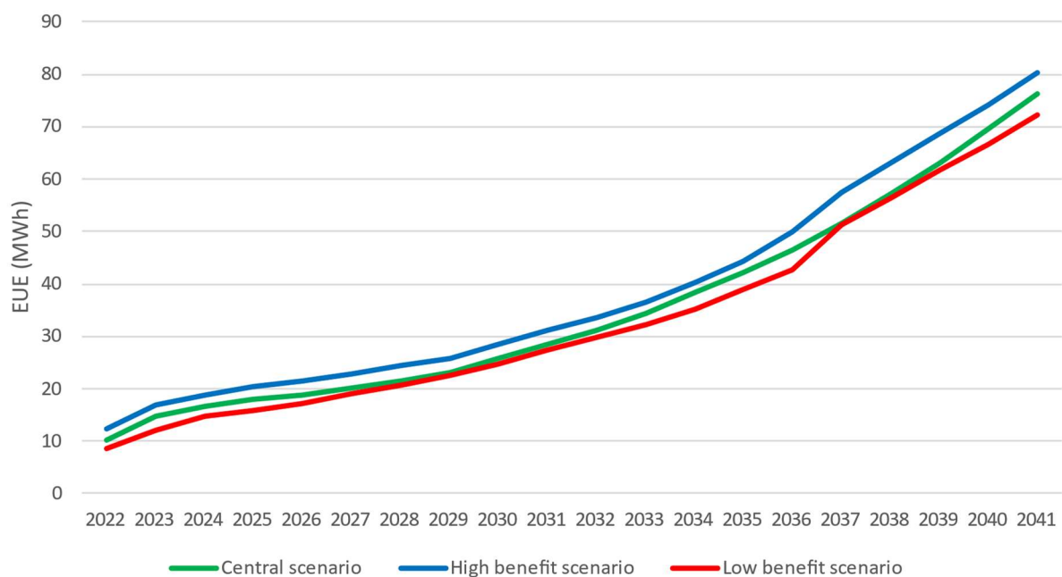
Figure 2-2 – Expected Unserved Energy forecasts for feeders 260 and 261
