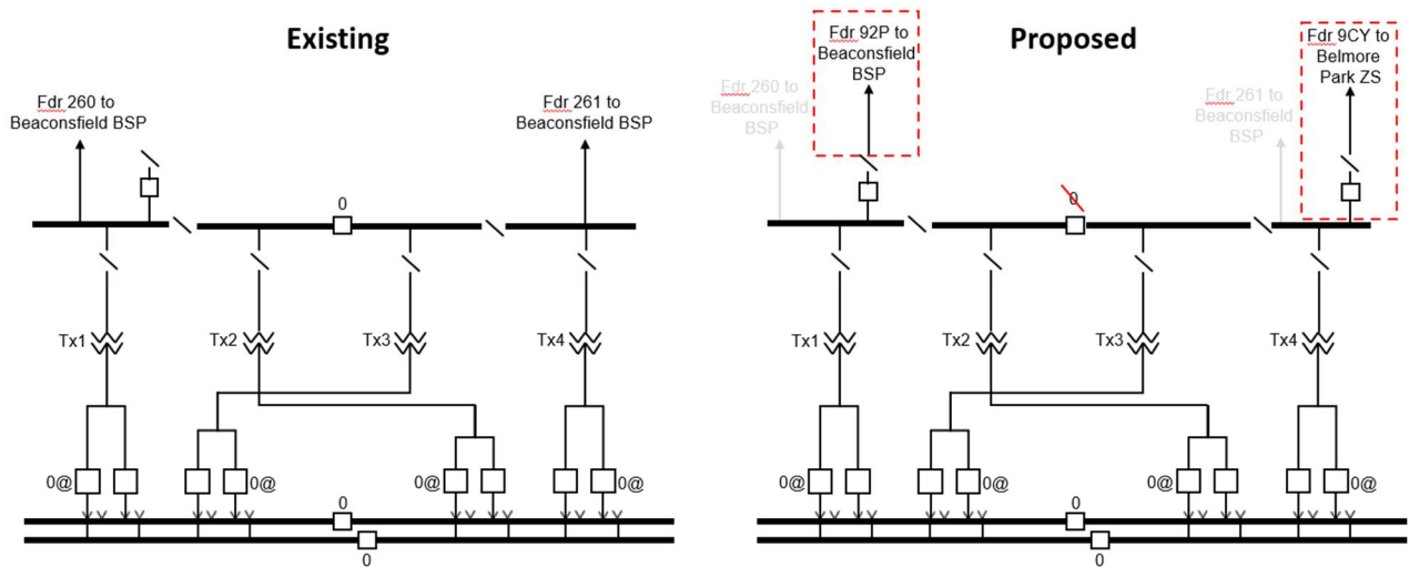
Figure 3-3 Existing and proposed diagram of Zetland ZS under Option 2
