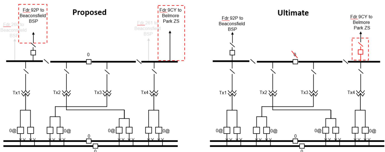
Figure 3-4 Diagram of proposed works at Zetland ZS under Option 3
