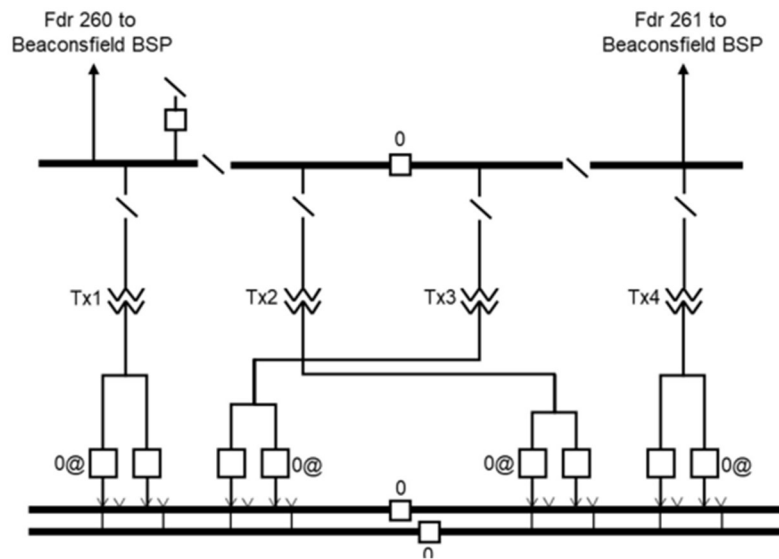
Figure 3-1– Diagram of existing Zetland ZS
