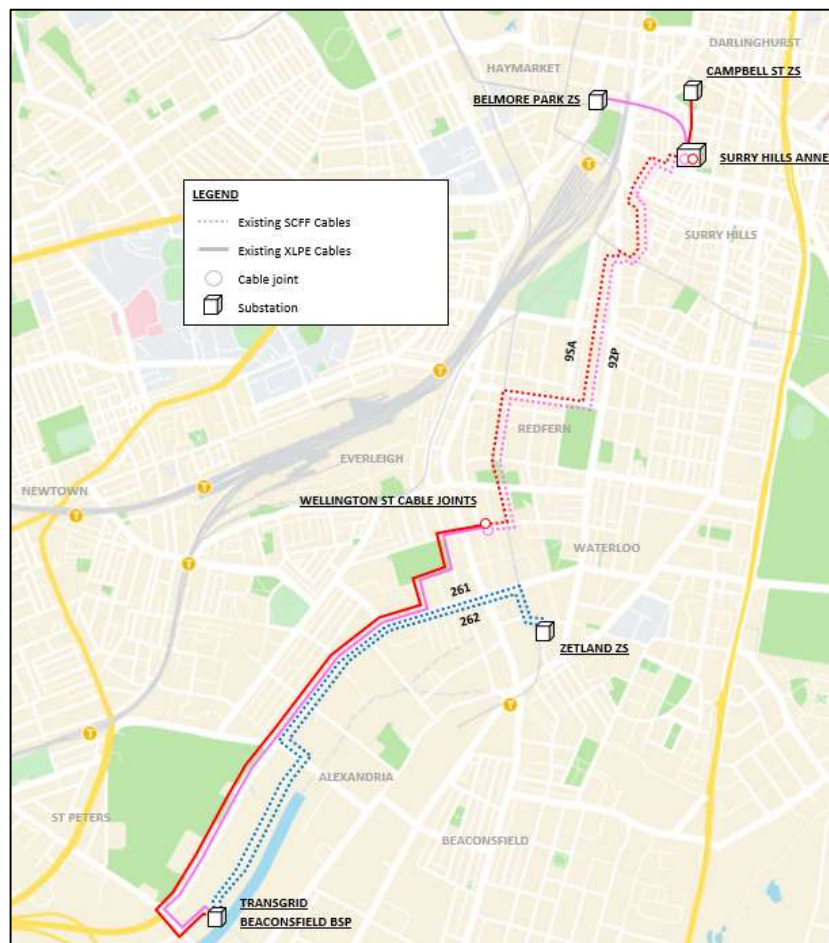
Figure 2-1 – Schematic view of the 132kV network including feeders 260, 261, 9SA and 92P
