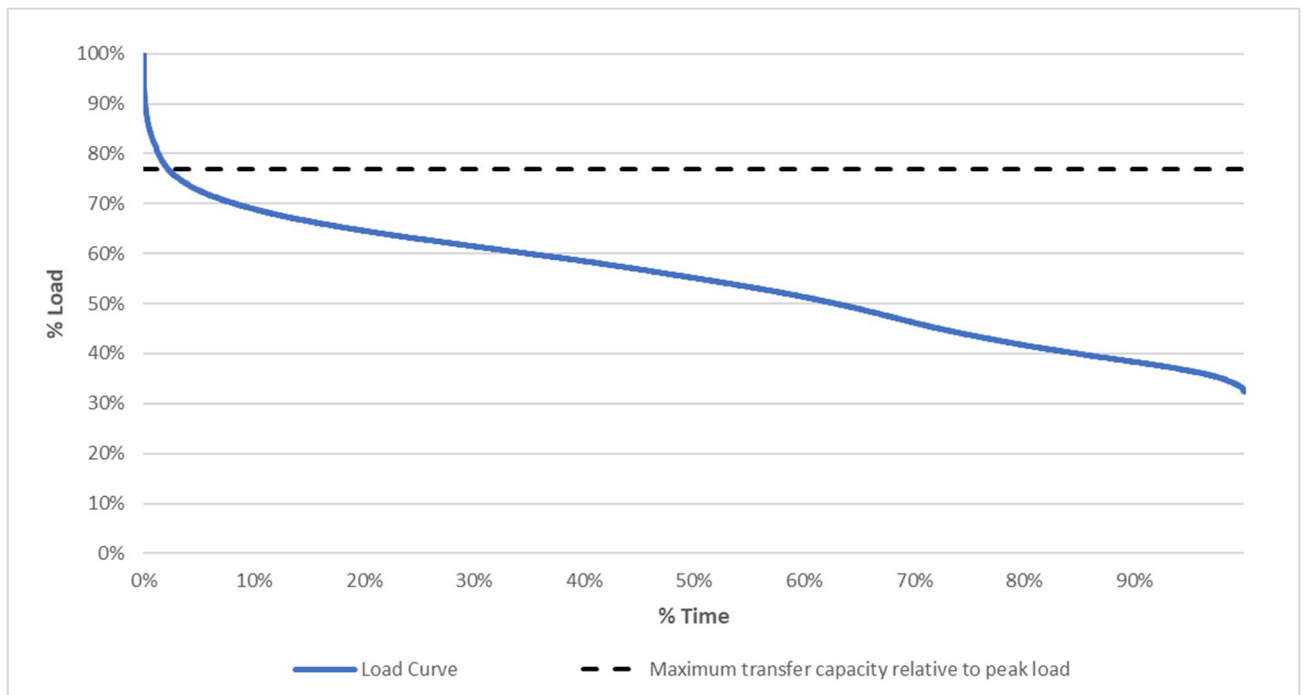
Figure D.1 – Load duration curve
