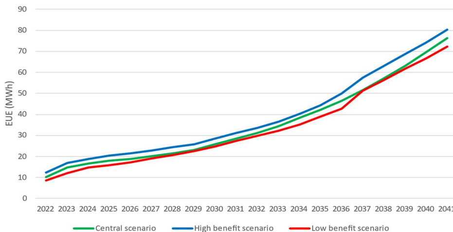
Figure 4-1 – Assumed expected unserved energy (EUE) under each of the three demand forecasts
