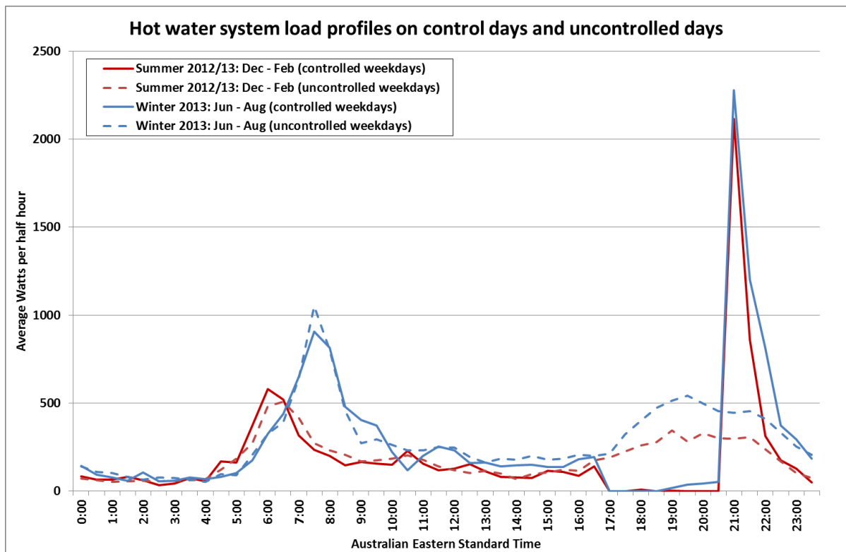
Figure 10: Averaged hot water system load profiles for 17 customers in the trial
