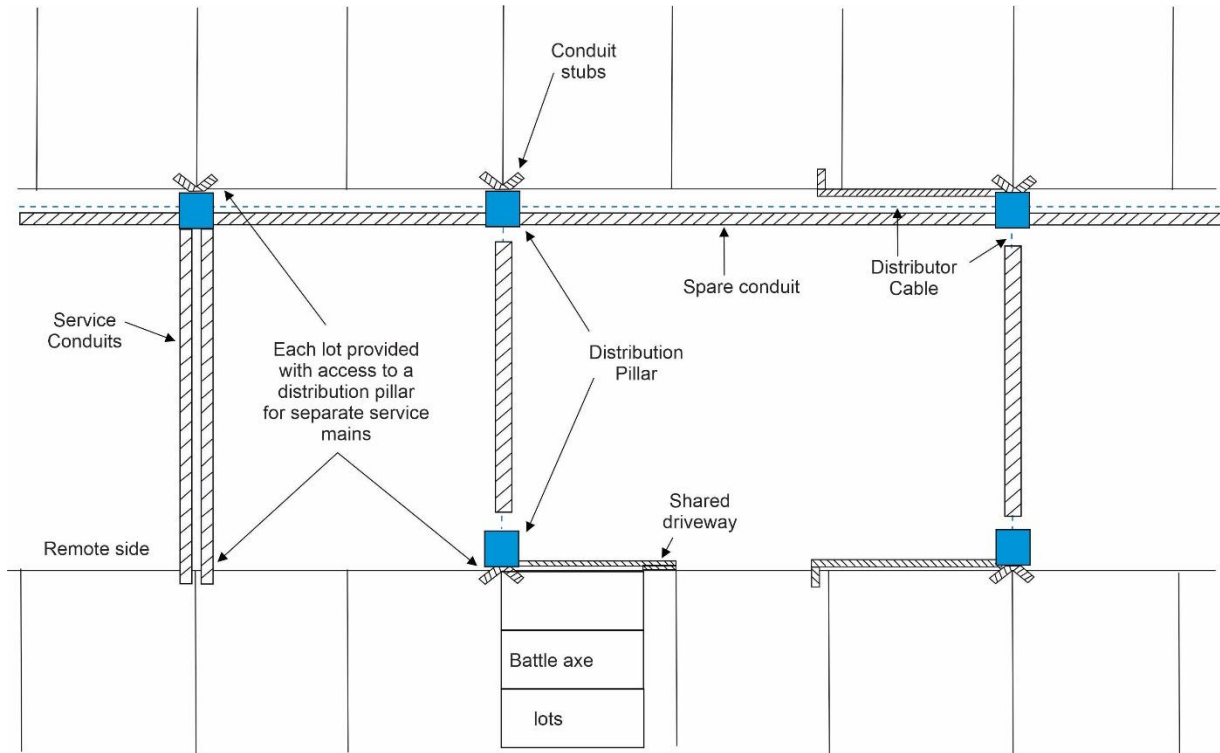
C2 LV distributor on both sides of the street
